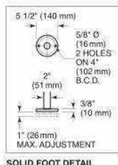
SOLID FOOT DETAIL
